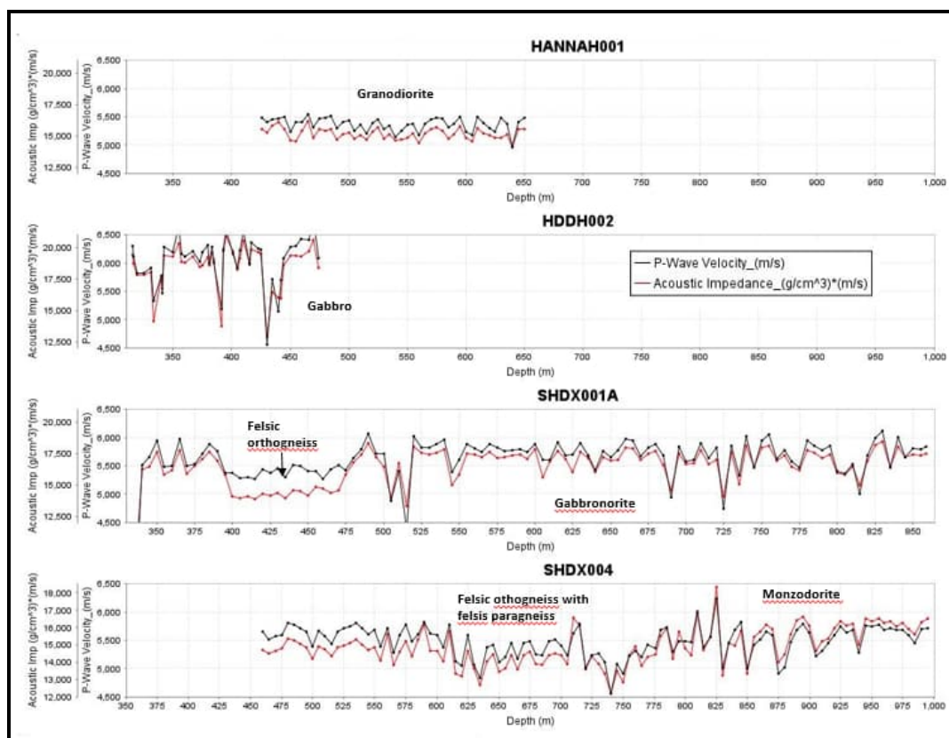
Figure 4 P-wave velocity & acoustic impedance for basement sequence of drill holes Hannah001, HDD002, SHDX001A, SHDX004.
