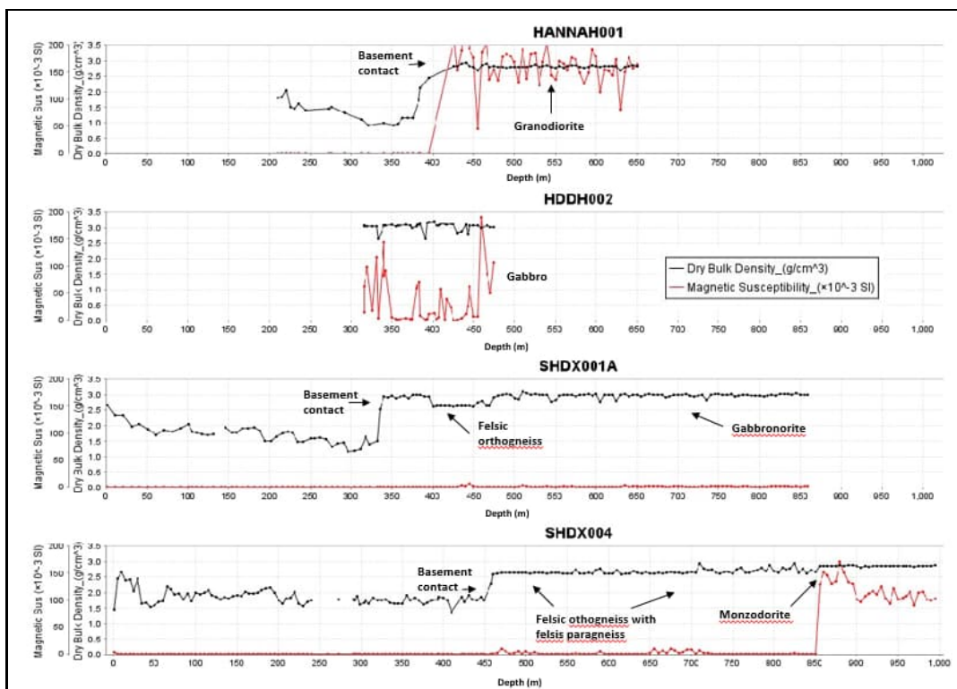
Figure 3 Dry bulk density and magnetic susceptibility data from drill holes Hannah001, HDD002, SHDX001A, SHDX004.
